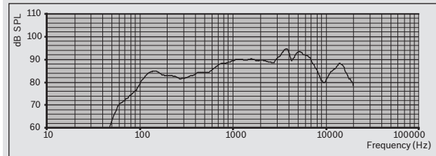
Frequency response
